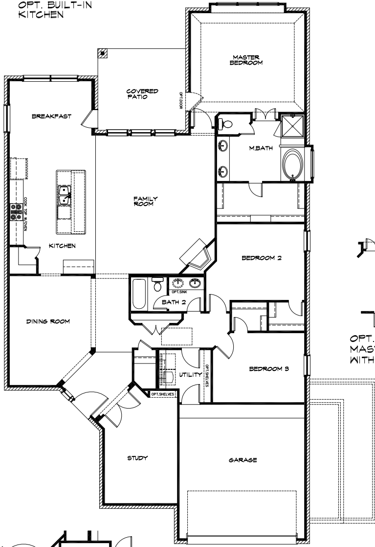
STANDARD 1ST FLOOR PLAN
