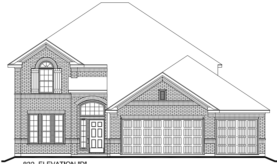
832 ELEVATION "D"
