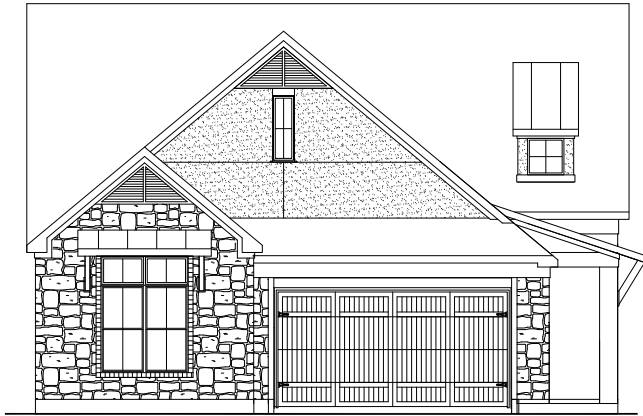
2224- ELEVATION "A"
