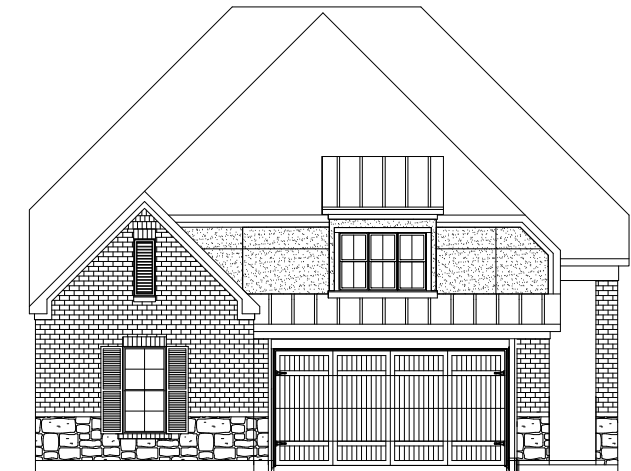
2224 - ELEVATION "C"
