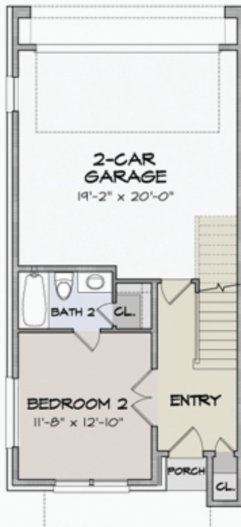
First Floor
