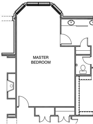
OPT BAY WINDOW @ MASTER BEDROOM
