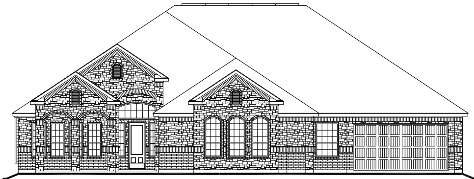
3522 ELEVATION "C"
