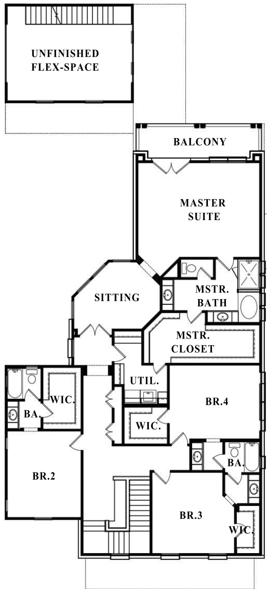
SECOND FLOOR
