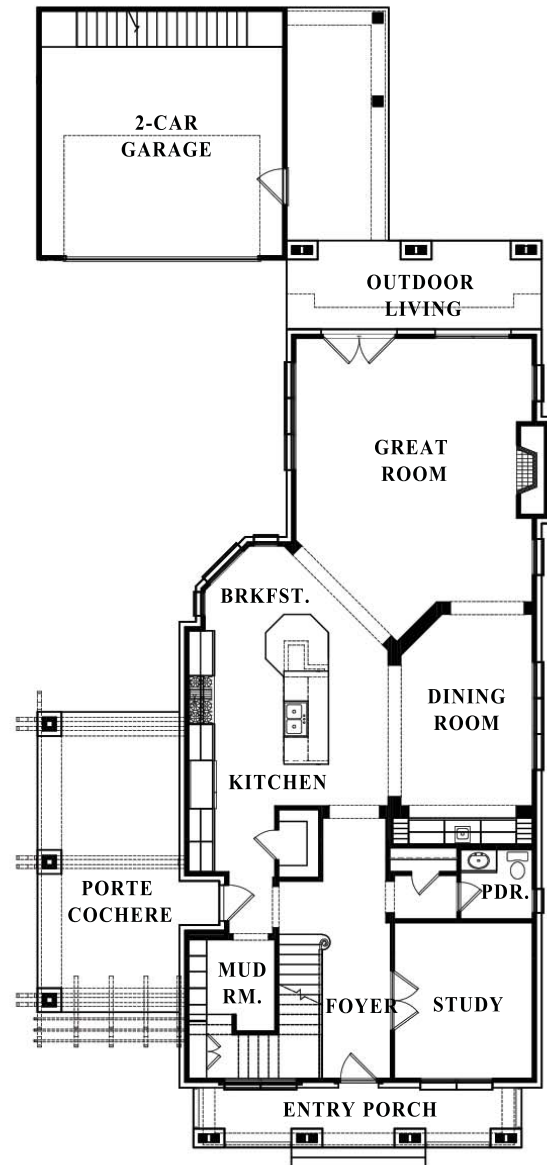
FIRST FLOOR
