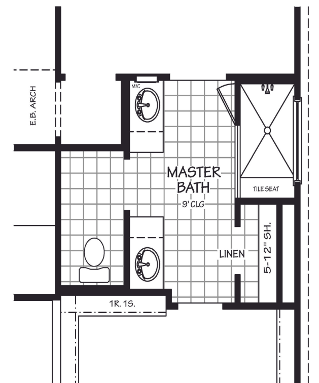
OPTIONAL MASTER BATH #3
