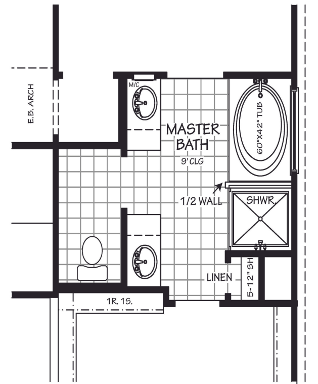
OPTIONAL MASTER BATH #1
