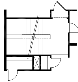
2ND FLOOR PLAN W/ 3RD FLOOR STAIR
