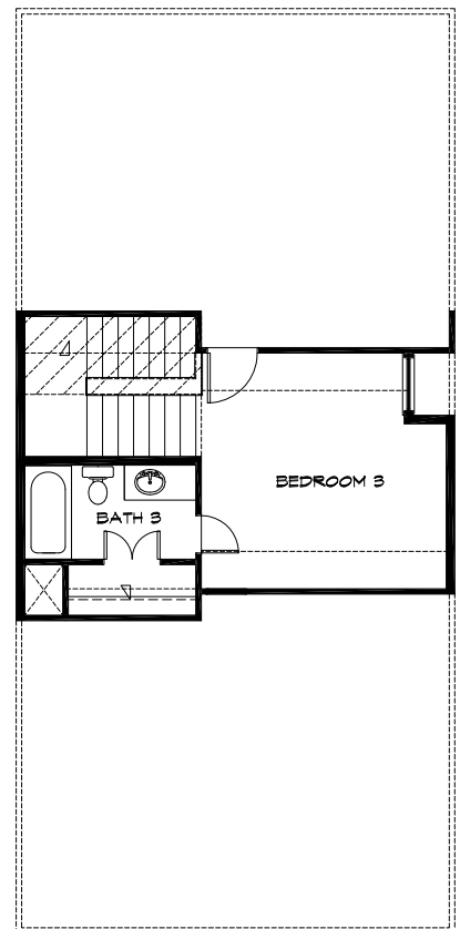
3RD FLOOR PLAN OPT.BEDROOM 3
